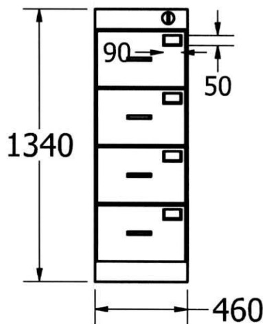
VISTA FRONTAL
